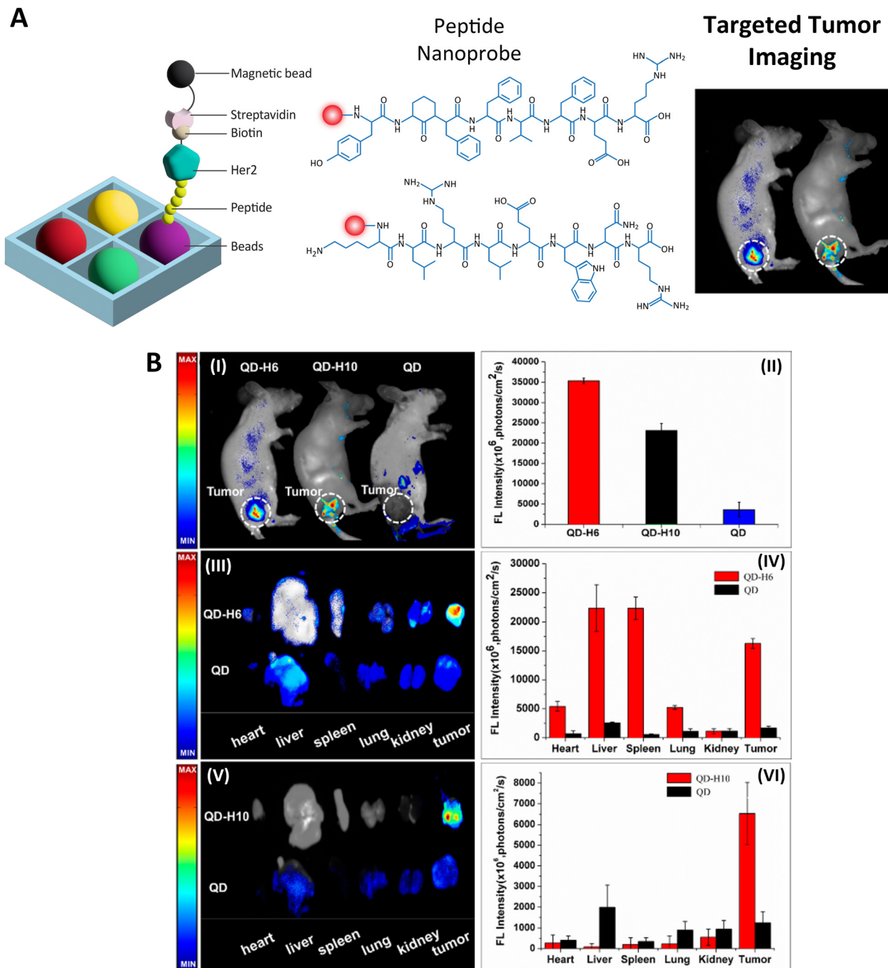
Fig. 20 (A) A diagram showing two newly found peptides, H6 (YLFFVFER) and H10 (KLRLWNR), which have a KD of 10 −8 M and display a strong affinity for the HER2 tumor biomarker. These peptides were extracted using a screening approach from a library of 10 5 peptides. When conjugated to NPs in vivo , H6 and H10 probes predominantly accumulated in HER2-positive tumor tissues of xenografted mice. Using H6-QD and H10-QD probes, in vivo and ex vivo imaging of tumors in mice was performed. Imaging in vivo with fluorescence (I, II) revealed the accumulation of peptide probes in malignancies. Experiments involving biodistribution and ex vivo fluorescence imaging were conducted on tumor-bearing null mice that had been dissected. After quantifying the fluorescence signals from ex vivo experiments, the mean fluorescence intensity of three separate observations was calculated. Reproduced from ref. 244 with permission from [American Chemical Society], copyright [2015].
