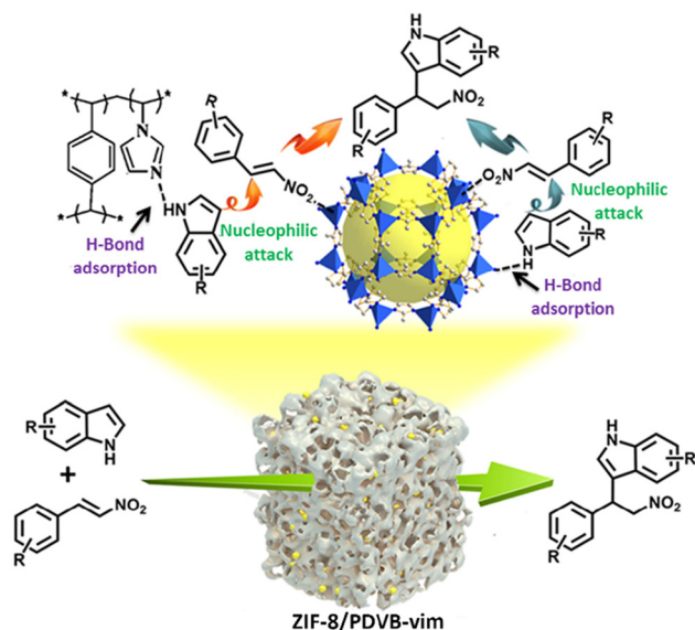
Scheme 1 The possible mechanism for the Friedel–Crafts reaction of indole with trans -β-nitrostyrene catalyzed by the ZIF-8/PDVB-vim composite.
