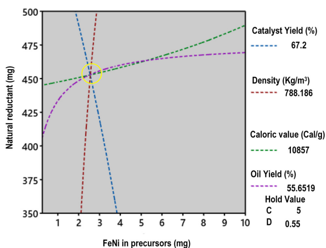
Fig. 9 Overlapping contour plots of oil yield. Calorific value and nano-catalyst yield, which result in the optimization point.
