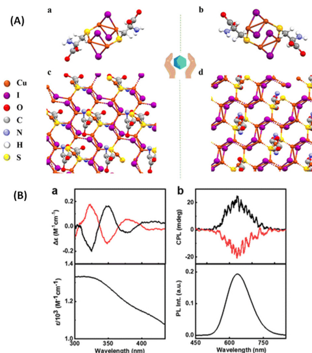
Fig. 12 (A) X-ray crystal structure of (a) (\text{D-Cys})_2\text{Cu}_4\text{I}_4 and (b) (\text{L-Cys})_2\text{Cu}_4\text{I}_4 nanoclusters and (B) experimental CD spectra (a) along with the corresponding absorption plot, and experimental CPL spectra (b) along with the corresponding luminescence spectra of the aqueous solution of nanoclusters. Black and red traces correspond to spectra collected from (\text{D-Cys})_2\text{Cu}_4\text{I}_4 and (\text{L-Cys})_2\text{Cu}_4\text{I}_4 nanoclusters, respectively. (Reproduced from ref. 51 with permission from the Royal Society of Chemistry, Copyright 2023).
