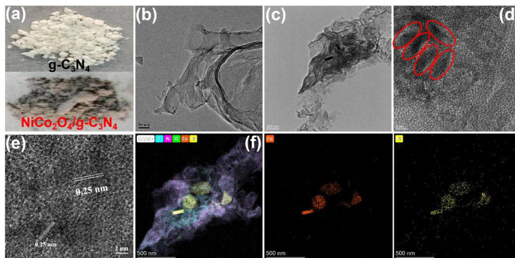
Fig. 2 Optical photos (a) and TEM images of g-C 3 N 4 nanosheets and NiCo 2 O 4 /g-C 3 N 4 composites at different magnifications (b–d), HRTEM image (e) of NiCo 2 O 4 /g-C 3 N 4 composites and the corresponding elemental mapping (f).
