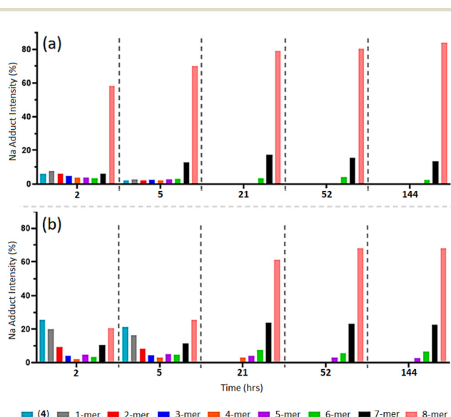
Fig. 6 MALDI-TOF mass spectra of multi-mer species [ n -mer + Na] + adduct intensities (relative percentages (%)) of timed “clicks” using 4.0 eq. CuSO 4 and 4.4 eq. Na ascorbate at 2, 5, 21, 52 and 144 h between (2a) and (4) (a) (full spectra shown in ESI S40–S47†), and between (2b) and (4) (b). (Full spectra shown in ESI S67–S71.†)
