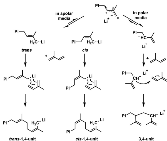
Scheme 2 Proposed mechanism of the polymerization of isoprene with lithium as a counter ion in apolar or polar media, respectively; image is reproduced from Frey et al. 41 with permission of the Royal Society of Chemistry, 2022.
