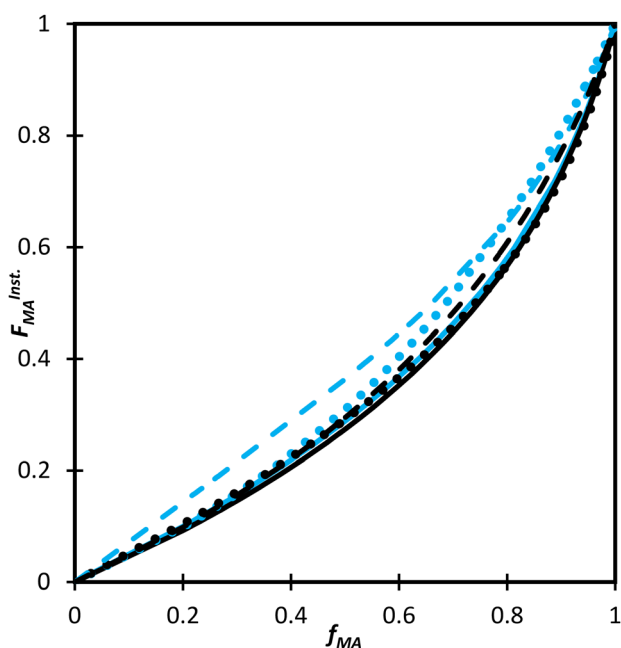
Fig. 9 F_{\text{MA}}^{\text{Inst.}} vs. f_{\text{MA}} calculated for the copolymerization of: MA/MAA (blue) and MA/DEGMEMA (black) in D 2 O : EtOD ( \alpha_{\text{EtOD}} = 0.5 ) (solid line) and in DMSO- d_6 with w_{\text{mon},0} = 0.50 (dots) and w_{\text{mon},0} = 0.10 (dashed). \alpha_{\text{EtOD}} refers to wt% of EtOD in D 2 O : EtOD mixture.
