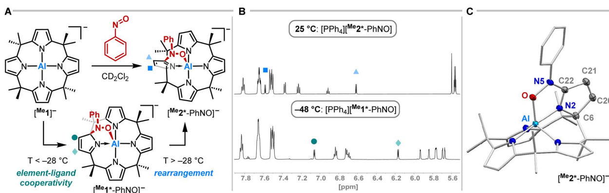
Fig. 4 (A) Synthetic scheme for the reaction of [\text{PPh}_4][^{\text{Me}}\mathbf{1}] with nitrosobenzene in dependence of the temperature. The tetraphenylphosphonium counterion is omitted for clarity. (B) ^1\text{H} NMR spectra (600 MHz, \text{CD}_2\text{Cl}_2 ) of the aromatic section of [\text{PPh}_4][^{\text{Me}}\mathbf{1}^*\text{-PhNO}] (bottom) and [\text{PPh}_4][^{\text{Me}}\mathbf{2}^*\text{-PhNO}] (top). (C) Solid state molecular structure of [\text{PPh}_4][^{\text{Me}}\mathbf{2}^*\text{-PhNO}]^- as determined by SCXRD analysis. The tetraphenylphosphonium counterion and all hydrogen atoms are omitted for clarity. Thermal displacement ellipsoids are displayed at the 50% probability level. Selected bond lengths [pm]: Al–O: 188.40(7), O–N5: 140.47(10), N5–C22: 135.28(12), C21–C22: 147.48(13), C20–C21: 134.27(14), C6–C20: 152.01(13), C6–N2: 143.94(12), N2–C22: 129.34(11). Selected bond angles [ ^\circ ]: Al–O–N5: 113.77(5), O–N5–C22: 112.88(7).
