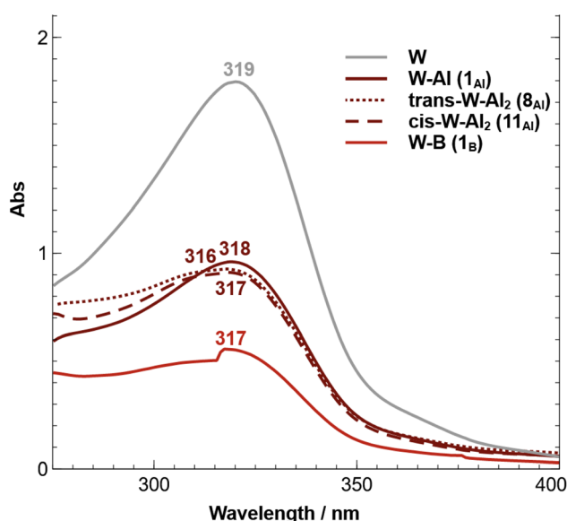
Fig. 9 Absorption spectra of trans-[W(depe)_2(N_2)_2] (W, grey line), trans-[W(depe)_2(N_2)(\mu-N_2-Al(C_6F_5)_3)] (W-Al, crimson line), trans-[W(depe)_2(\mu-N_2-Al(C_6F_5)_3)_2] ( trans-W-Al_2 , dotted crimson line), cis-[W(depe)_2(\mu-N_2-Al(C_6F_5)_3)_2] ( cis-W-Al_2 , dashed crimson line), and trans-[W(depe)_2(N_2)(\mu-N_2-B(C_6F_5)_3)] (W-B, red line). The concentration of each sample is about 30\text{ }\mu\text{M} .
