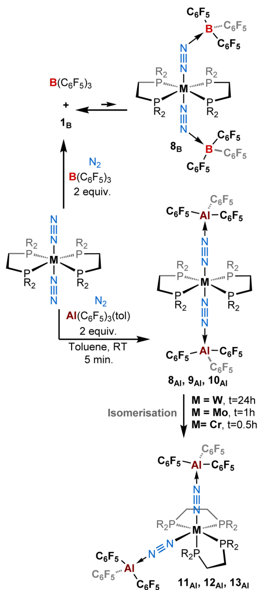
Scheme 3 Reactivity of [ML_2(N_2)_2] ( M = W, Mo, Cr ; L = depe, dppe, dmpe ) complexes with (top) two equivalents of B(C_6F_5)_3 and (bottom) two equivalents of Al(C_6F_5)_3(tol) under a dinitrogen atmosphere.
