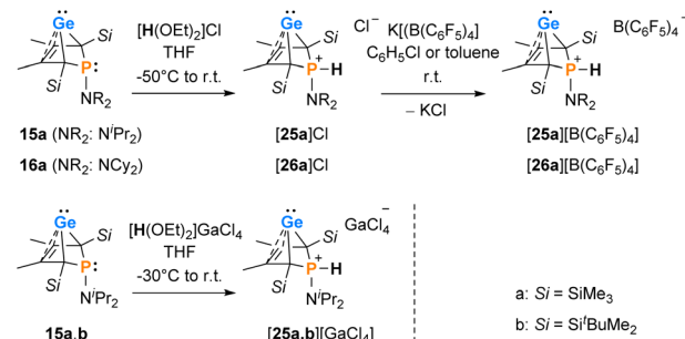
Scheme 2 Protonation of phospho-BCHGe's 15 , 16 .
