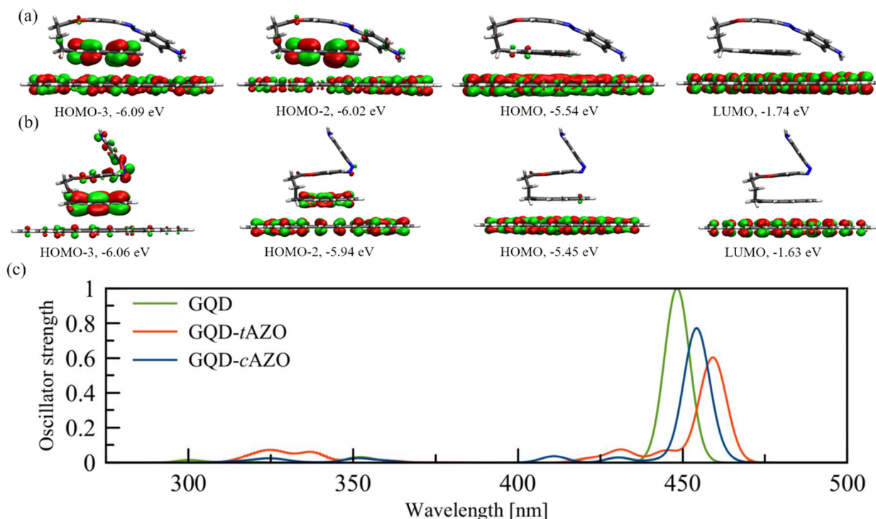
Fig. 3 Frontier orbitals of (a) GQD-tAZO and (b) GQD-cAZO. (c) UV-Vis spectra of GQD-tAZO interfaces (red and blue lines) and GQDs (green line).
