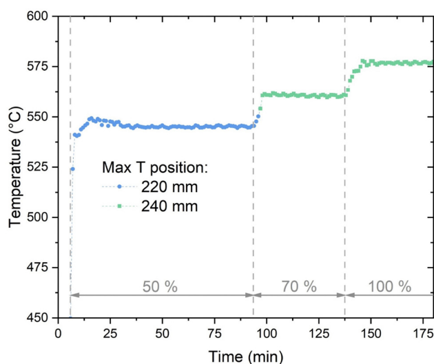
Fig. 3 The evolution of the maximum temperature in the methanation reactor (experimental conditions: 8 bar, H_2 : CO_2 = 4.15 , cooling setpoint = 230\text{ }^{\circ}\text{C} ).
