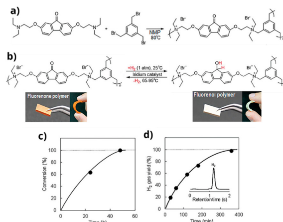
Fig. 9 (a) Synthesis of fluorenone polymer, (b) dehydrogenated and hydrogenated forms of fluorenone (orange)-fluorenel (white) polymer sheets, (c) hydrogenation kinetics of fluorenone polymer at 25 °C and 1 atm of hydrogen gas and (d) dehydrogenation kinetics of fluorenel polymer at 95 °C (inset gas chromatography plot of the hydrogen peak). 52 Copyright Wiley 2020.
