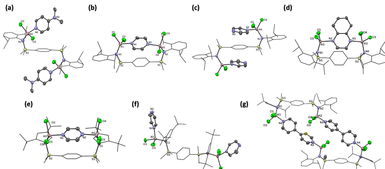
Fig. 2 ORTEP diagram showing the molecular structures of (a) 1-(DMAP) 2 , (b) 1-κ 2 -pyz, (c) 1-(pyz) 2 , (d) 1-κ 2 -quil, (e) 2-κ 2 -pyz, (f) 2-(pyz) 2 , and (g) 12-μ-(bipy) 2 (thermal ellipsoids drawn at the 50% probability level for Al, C, Si, N, and O; capped sticks representation for the ligand skeleton; H atoms have been omitted for clarity).
