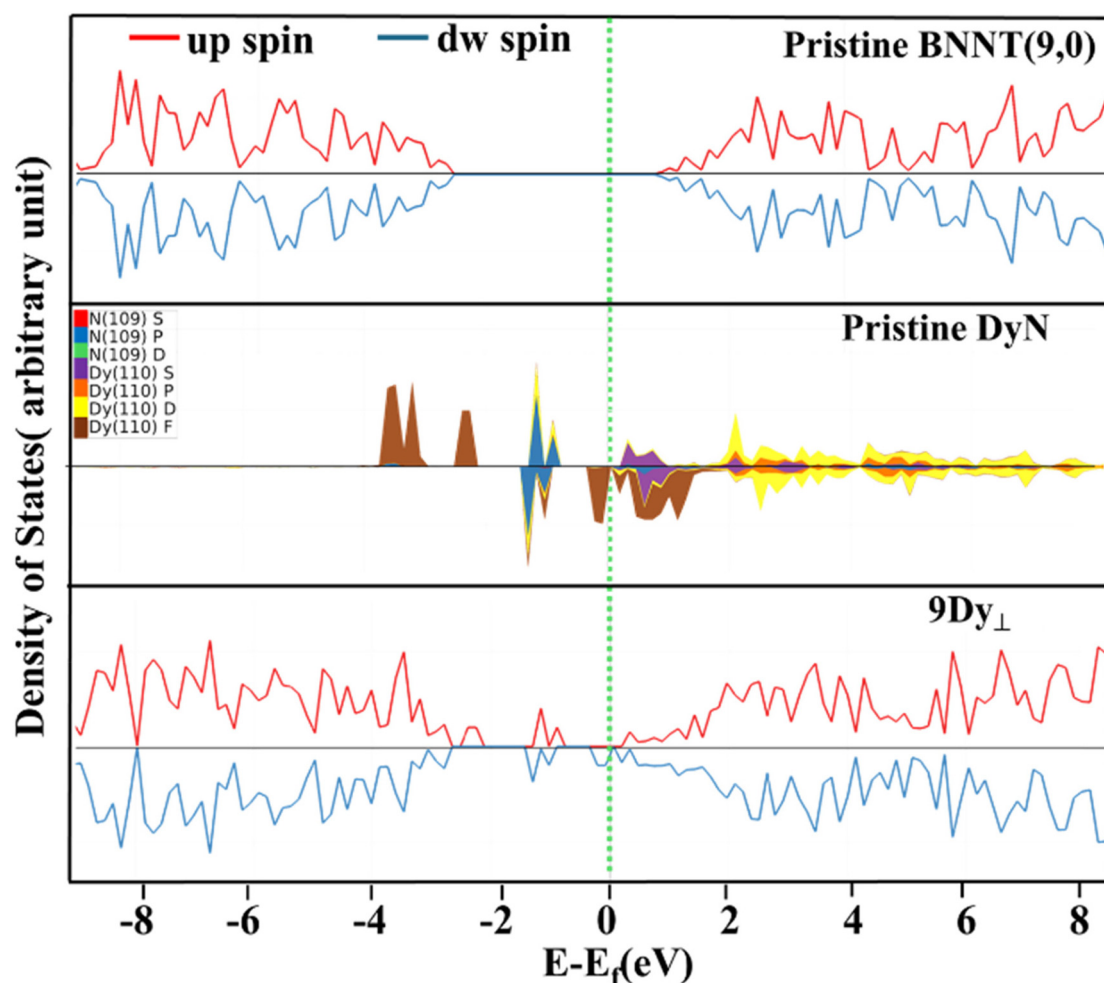
Fig. 3 Density of States plot for 9Dy ⊥ . The green dotted line shows the Fermi level.
