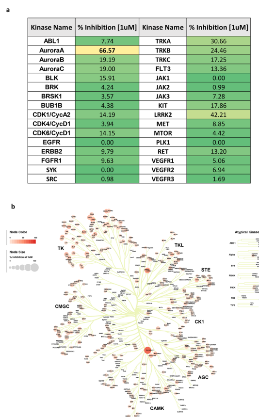
Fig. 9 Kinase inhibition profile of lead 2D7 . a ) Summary of kinase profiling. Table shows the percentage of enzymatic inhibition after treatment with 1 \mu\text{M} of 2D7 , the mean percentage are respect to DMSO control. Colour scale highlights the inhibition percentage values from the lowest (green) to the highest (red). b ) Kinome phylogenetic tree showing the selectivity of compound 2D7 for the Aurora kinase A over a panel 340 protein kinases. Note that only kinases listed on Coral software 44 were used for this plot. The size of the dots is relative to the mean percentage (%) of inhibition to the corresponding kinase at a dose of 1 \mu\text{M} . Where dots are not present, the kinase was not evaluated.
