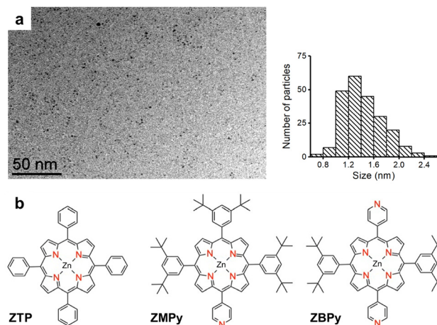
Fig. 1 (a) TEM picture and size distribution of the pristine ultra-small ( 1.4 \pm 0.3 nm) Pt NP; (b) chemical structure of the ZTP, ZMPy and ZBPpy porphyrins.
