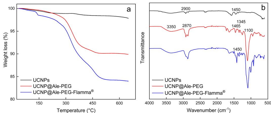
Fig. 3 (a) TGA thermograms and (b) FTIR spectra of UCNPs, UCNP@Ale-PEG and UCNP@Ale-PEG-Flamma® particles.
