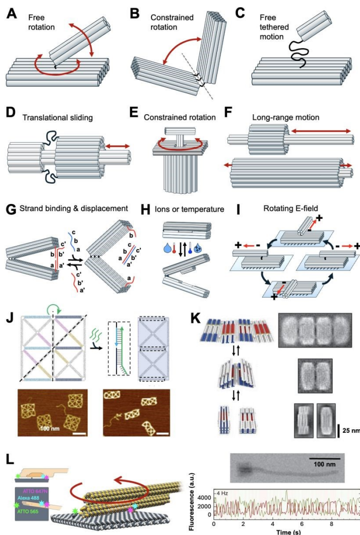
Figure 1: Dynamic mechanisms in DNA origami structures. (A-F) Strategically placed ssDNA connections can produce a diverse range of motions: (A) free rotation about a point, (B) rotation constrained to a single angular degree of freedom, (C) free motion through tethers, (D) translational sliding through interlocked structures, (E) rotary motion constrained by concentric structures with an end cap on the outer structure, and (F) long-range translational sliding along tracks. (G-I) Various actuation methods can be used to control motion: (G) toehold-mediated strand displacement, (H) environmental triggers such as temperature or ion concentration, and (I) electric fields. (J-L) Experimental examples of dynamic DNA origami structures: (J) sheets that fold along different lines in response to different ssDNA trigger strands, (K) a sheet that reversibly folds into blocks using salt-dependent shape-complementary base stacking interactions, and (L) electric-field driven DNA origami rotor. Panels J, K, and L have been adapted with permission from ref. 25 (Copyright 2023, Springer Nature), ref. 22 (Copyright 2015, AAAS), and ref. 12 (Copyright 2018, AAAS), respectively.
