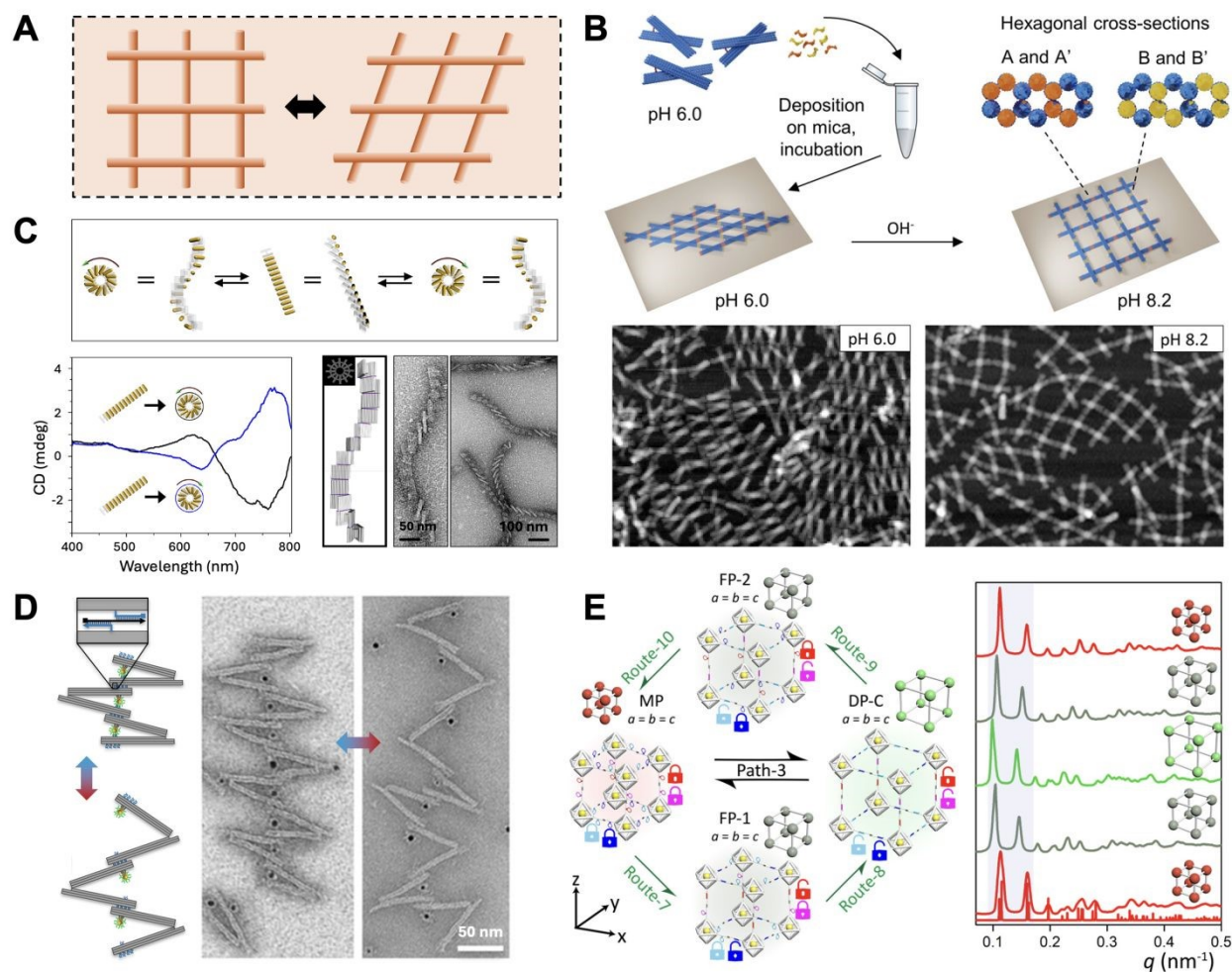
Figure 4: Reconfigurable superstructures assembled from dynamic origami building blocks. (A) Schematic of a reconfigurable lattice. (B) Accordion-like reconfiguration of an origami assembly in response to changes in pH (reproduced with permission from ref. 59; Copyright 2023 American Chemical Society). (C) Linear array of origami-nanoparticle assemblies that switch chirality after addition of trigger strands (reproduced with permission from ref. 56; Copyright 2018 American Chemical Society). (D) Origami-nanoparticle chains that can rapidly cycle between two states at different temperatures (reproduced with permission from ref. 58; Copyright 2019 American Chemical Society). (E) Crystals of nanoparticle-carrying origamis with changeable lattice parameters and the corresponding SAXS spectra for each lattice type (reproduced with permission from ref. 63; Copyright 2023 American Chemical Society).
