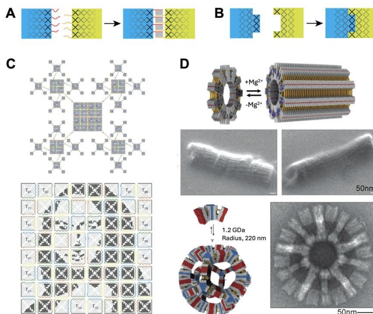
Figure 2: Hierarchical assembly of DNA origami via (A) programmable sticky-end hybridization and (B) shape-matching blunt-end stacking. (C) Hierarchical assembly of large arrays, including a picture mimicking the painting of Mona Lisa, from DNA origami tiles (reproduced with permission from ref. 35; Copyright 2017, Springer Nature). (D) Hierarchical assembly of DNA-origami gigadalton structures, including a self-limiting nanotubes and 3D cages, via blunt-end stacking (reproduced with permission from ref. 38; Copyright 2017, Springer Nature).
