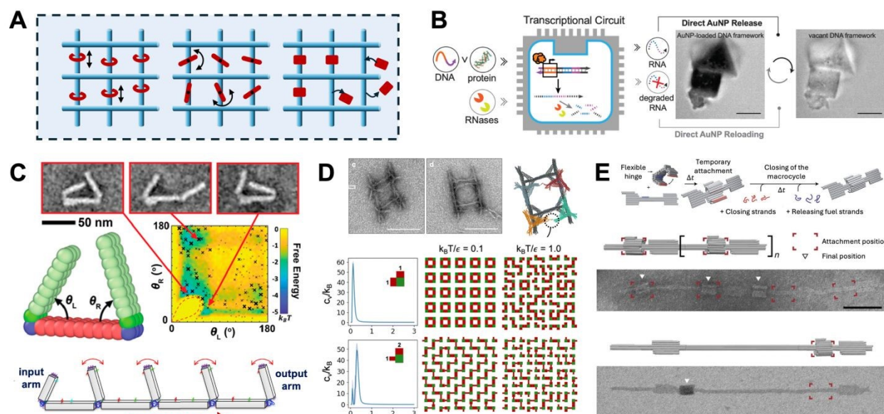
Figure 5: Static superstructures housing dynamic DNA origami subunits. (A) Schematic of such lattices with translatable, rotatable, and dissociable components. (B) Crystal that loads and unloads gold nanoparticles in response to the output of a transcriptional circuit (reproduced with permission from ref. 68; Copyright 2024, American Chemical Society). (C) TEM images and angle distributions from coarse-grained simulations of minimal unit of a sterically communicating DNA origami array (reproduced with permission from ref. 66; Copyright 2023, American Chemical Society). (D) TEM images of 2 \times 2 rotor lattice and order-disorder transitions of 10 \times 10 lattices as predicted by Monte Carlo simulations (reproduced with permission from ref. 67; Copyright 2023, Royal Society of Chemistry). (E) Method for assembling mechanically interlocked rotaxane-like structures, as well as TEM images showing movement of the dynamic component (reproduced with permission from ref. 16; Copyright 2016, Springer Nature).
