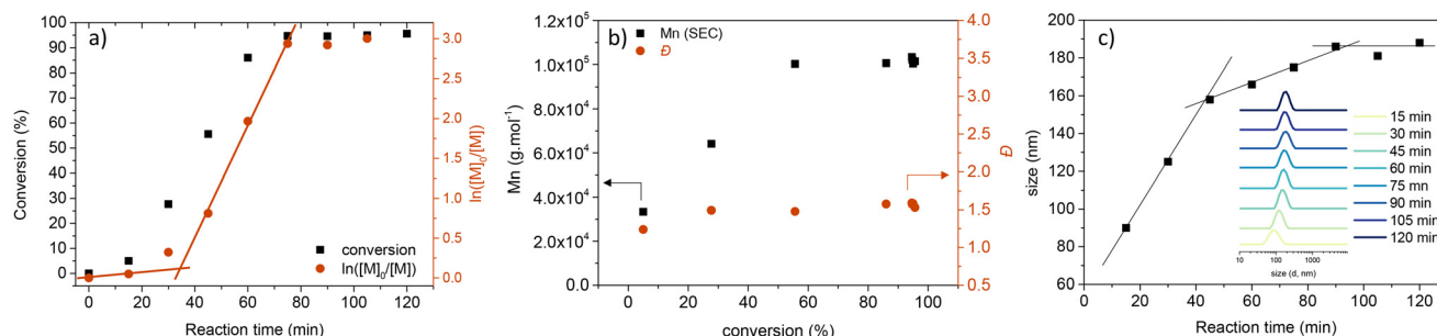
Fig. 4 Kinetics of chain extension of the P \epsilon LL 2.9k macroCTA with HPMA (DP 0 = 100) at 5 wt% in terms of (a) conversion over the reaction time and pseudo-first linear plot, (b) molar mass and polydispersity evolution from SEC measurements with the exclusion of non-functionalised P \epsilon LL residuals, and (c) size evolution of the formed nanoparticles over time by DLS measurement.
