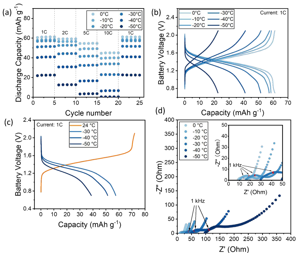
Figure 6. PNTCDI || PTMA- co -GMA full cell characteristics at low temperatures from -50 °C to 0 °C (a) Discharge capacity at current from 1C (110 mA g -1 ) to 10C (1100 mA g -1 ). (b) GCD profiles of the cell at 1C. (c) GCD curves for the cell battery charged at room temperature, kept at 2.1 V while cooling down, and then discharged at various low temperatures. (d) EIS Nyquist plot of the full cell at different temperatures.
