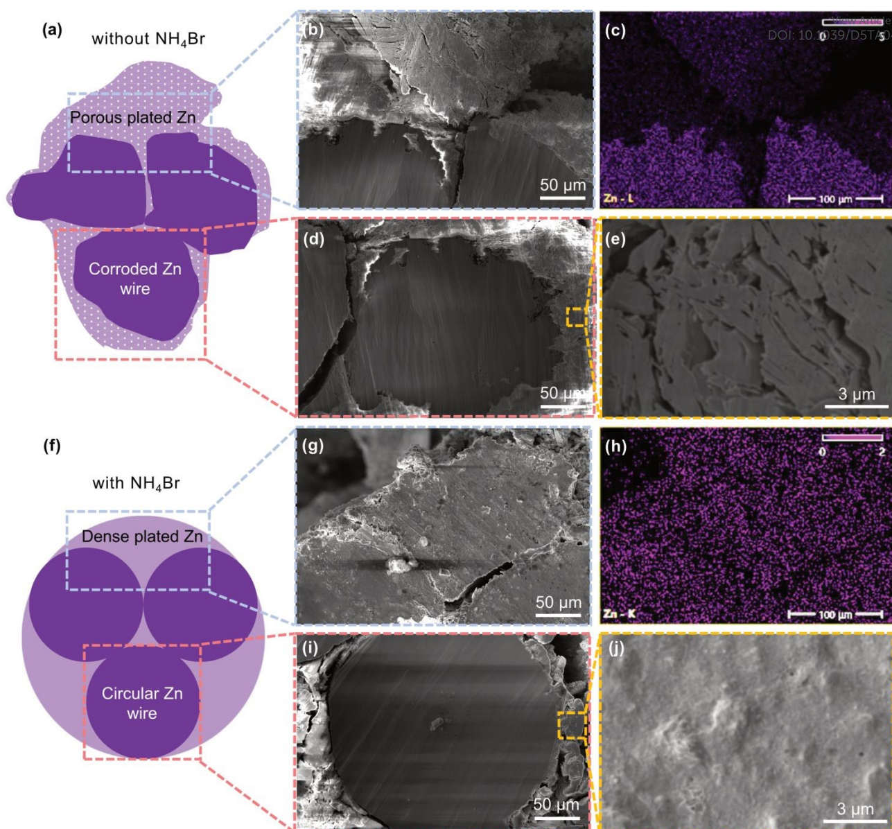
Figure 4. Postmortem analysis of Zn wire anodes cycled with and without \text{NH}_4\text{Br} . (a) Schematic of Zn wire after cycling without \text{NH}_4\text{Br} , with non-uniform and porous Zn plating and Zn wire corrosion. (b) Cross-sectional SEM image and (c) Zn elemental mapping of Zn plated between two Zn wires without additive. (d) SEM of Zn wire after cycling, with shape deformed and edge corroded. (e) Zoom-in image of plated Zn showing porous structure. (f) Schematic of Zn wire after cycling with \text{NH}_4\text{Br} , with uniform and dense Zn plating. (g) Cross-sectional SEM image and (h) Zn elemental mapping of Zn plated between two Zn wires with additive. (i) SEM of Zn wire after cycling, with circular shape retained and a smooth edge. (j) Zoom-in image of plated Zn showing dense structure.
