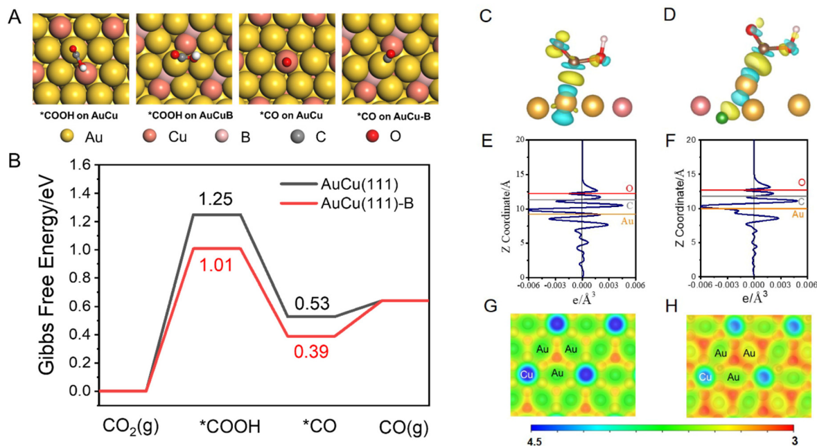
Fig. 5 (A) Adsorption configurations of \text{*COOH} and \text{*CO} on AuCu(111) and AuCu(111)-B. (B) Gibbs free energy profiles for \text{CO}_2\text{RR} on AuCu(111) and AuCu(111)-B. Charge density difference plots of \text{*COOH} adsorption on AuCu(111) (C) and AuCu(111)-B (D). Planar-averaged charge density difference of \text{*COOH} adsorption on AuCu(111) (E) and AuCu(111)-B (F). Surface electrostatic potentials of AuCu(111) (G) and AuCu(111)-B (H).
