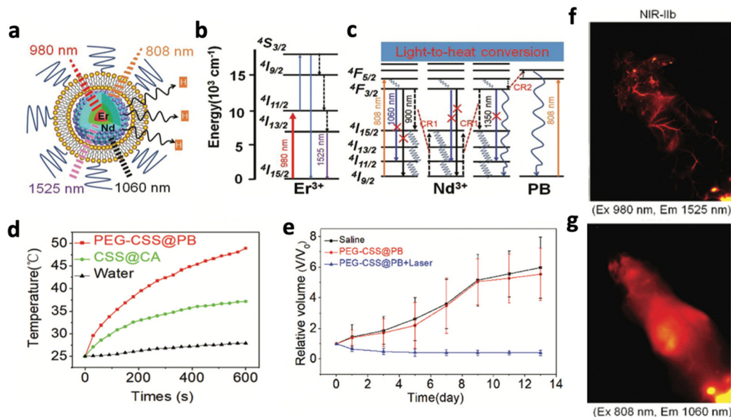
Fig. 16 Schematic illustrations of (a) the design of \text{NaErF}_4@\text{NaYF}_4@\text{NaNdF}_4 exhibiting NIR-II luminescence under orthogonal excitation, (b) energy transition diagrams of the 1525 nm luminescence of \text{Er}^{3+} under 980 nm excitation and (c) energy transition diagrams of the 1060 nm luminescence of \text{Nd}^{3+} under 808 nm excitation, with cross-relaxation pathways between \text{Nd}^{3+} ions and \text{Nd}^{3+} ions with PB. (d) Comparison of temperature increases of the PEG-CSS@PB nanocomposite, CSS@CA nanocomposite and water, excited by a 808 nm laser ( 1 \text{ W cm}^{-2} ). (e) Comparison of tumour volume following different groups of treatment. In vivo NIR II luminescence imaging of the mouse with a tail vein injection of PEG-CSS@PB, acquired with (f) 1525 nm and (g) 1064 nm luminescence. Reproduced with permission from ref. 65. Copyright 2019, Royal Society of Chemistry.
