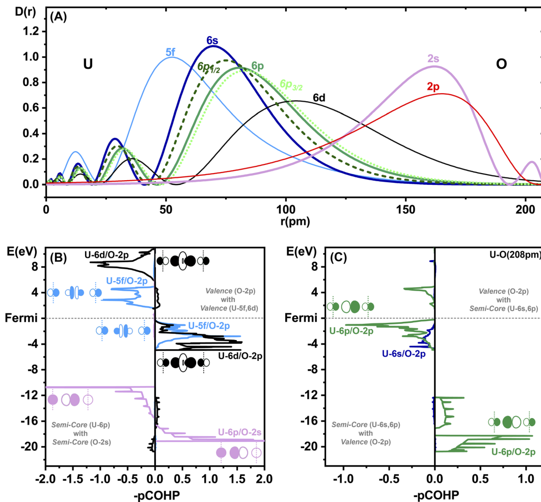
Fig. 3 Bonding analysis of \delta -[UO 3 ]. (Top) (A) Radial atomic orbital density distributions D(r) (in atomic units, ZORA-PBE density functional calcs.) of U^{6+} at r = 0 , and of O^0 at r = 208 (the U–O distance in \delta -[UO 3 ], r in pm). Fully occupied semi-core orbitals are bold: U-6s (solid, dark blue), spin-averaged U-6p (solid, green), SO split U-6p 1/2 (dashed, dark green) and U-6p 3/2 (dotted, light green). Valence orbitals are thin: inner U-5f (blue), outer U-6d (black). Orbitals of O, in reverse: O-2s (bold, lilac) and O-2p (thin red). (Bottom) Projected crystal orbital Hamilton populations (pCOHP) of \delta -[UO 3 ] in the semi-core & valence regions (SR-PBE approximation) calculated with LOBSTER. 51,52 Positive and negative values indicate, respectively, bonding and antibonding interactions, as shown by the AO sketches along an axis of the unit cell, with O atoms at the corners (vertical dashed lines) and the U atom in between. (Left) (B) At the top, the common dative valence interactions of O-2p into U-5f (blue) and U-6d (black), bonding below and antibonding above the Fermi edge; at the bottom, the 'degeneracy-driven' semi-core interactions due to the overlap of U-6p and O-2s (lilac). (Right) (C) The 'unusual' semi-core/valence interactions U-6s/O-2p (dark blue) and U-6p/O-2p (green), stabilizing the semi-core shells (at the bottom), and destabilizing (PFB) the valence levels in particular around the Fermi edge (at the top).
