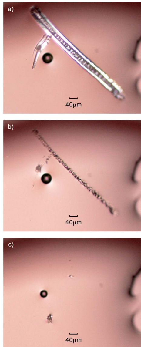
Fig. 7 Photos of (a) scratches made on the surface of the cross-linked epoxy polymer sample, (b) partially healed sample after heated at 140 °C for 30 minutes and (c) fully healed sample after heated at 140 °C for 30 minutes.
