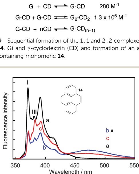
Fig. 7 Fluorescence spectra for pyrene ( 14 , 0.5 \mu\text{M} ) in water (a, black) and in the presence of 5 mM (b, blue) and 20 mM (c, red) \gamma -cyclodextrin. (Adapted with permission from A. S. M. Dyck, U. Kisiel and C. Bohne, J. Phys. Chem. B , 2003, 107 , 11652–11659. Copyright 2003 American Chemical Society.)
