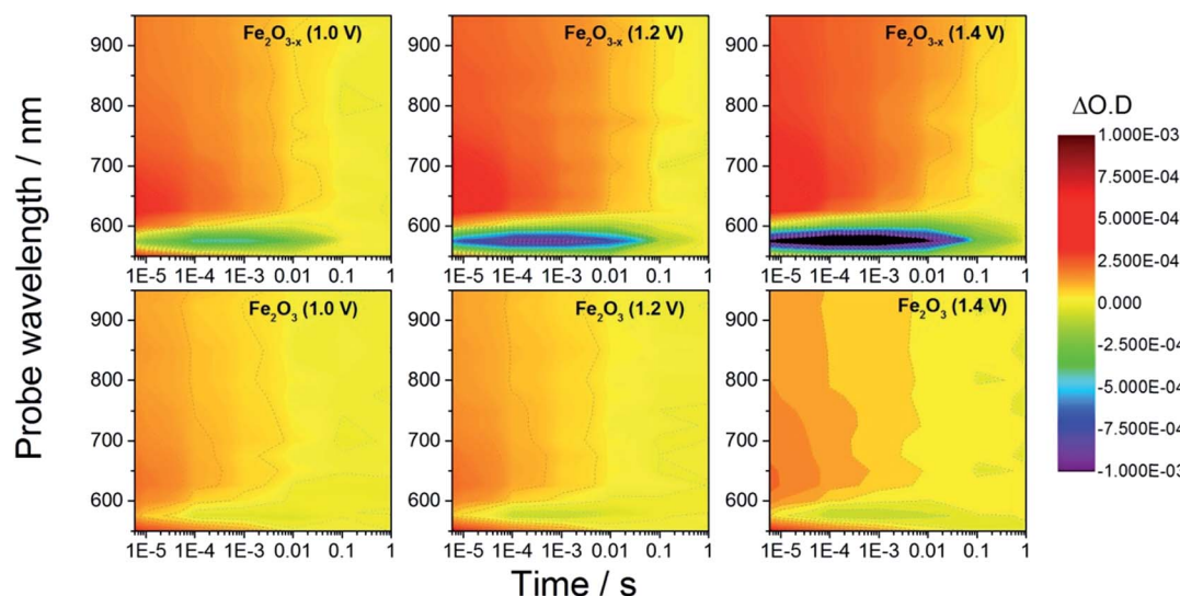
Fig. 2 TA spectra of \alpha\text{-Fe}_2\text{O}_3 and \alpha\text{-Fe}_2\text{O}_{3-x} at various applied potentials (vs. RHE) in 1 M NaOH with the photoanodes excited from the electrolyte/electrode side (EE) with a 355 nm (6 ns pulse) laser.
