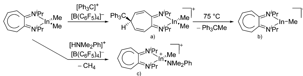
Fig. 25 Formation of tetra- and tricoordinate cationic diimine substituted indium complexes: (a) [(^i\text{Pr}_2\text{-ATl}(\text{CPh}_3))\text{InMe}_2]^+ , (b) [(^i\text{Pr}_2\text{-ATl})\text{InMe}]^+ and (c) [(^i\text{Pr}_2\text{-ATl})\text{In}(\text{Me})(\text{NMe}_2\text{Ph})]^+ . For each complex, the counterion is [\text{B}(\text{C}_6\text{F}_5)_4]^- .
