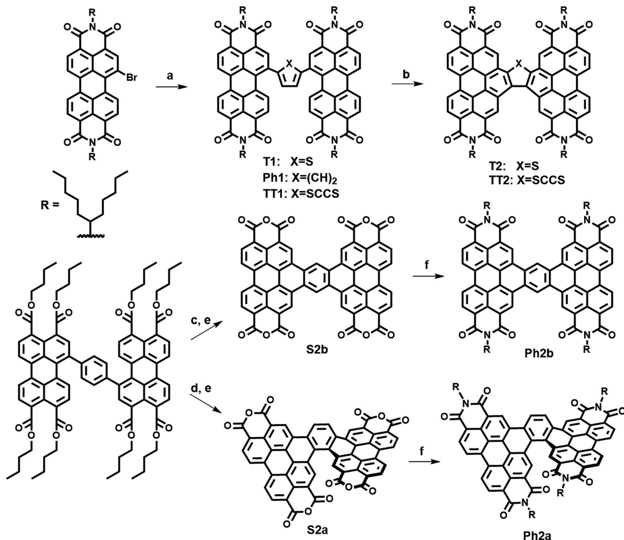
Scheme 1 Synthesis of PDI dimers. (a) Pd(PPh 3 ), toluene, (84–90%) (b) hv , toluene, air (84–88%) (c) CH 2 Cl 2 , I 2 , air, hv (d) (1) toluene, I 2 , hv , N 2 (2) DDQ (e) ClSO 3 H (65–78% over 2 steps) (f) imidazole, 1-pentylhexyl.
