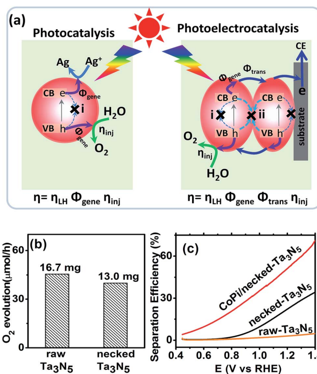
Fig. 4 (a) Schematic comparison of O 2 evolution processes via photocatalysis (AgNO 3 as electron scavenger) and photoelectrocatalysis. (b) Photocatalytic activity of the Ta 3 N 5 powder peeled from raw-Ta 3 N 5 and necked-Ta 3 N 5 electrodes. The mass of the photocatalyst is listed above the column, respectively. (c) Charge separation efficiency of raw-Ta 3 N 5 (orange), necked-Ta 3 N 5 (black) and CoPi/necked-Ta 3 N 5 electrodes (red).
