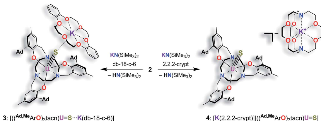
Scheme 2 Synthesis of the terminal uranium(IV) sulfido complexes [(\text{Ad,MeArO})_3\text{tacn}]\text{U}\equiv\text{S}\cdots\text{K}(\text{db-18-c-6}) ( 3 ) and [\text{K}(2.2.2\text{-crypt})][[(\text{Ad,MeArO})_3\text{tacn}]\text{U}\equiv\text{S}] ( 4 ).
