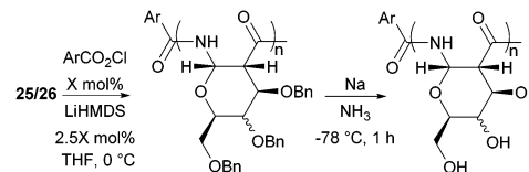
Fig. 25 Anionic ROP of \beta -lactam sugar monomers and subsequent benzyl deprotection with sodium metal in ammonia.
