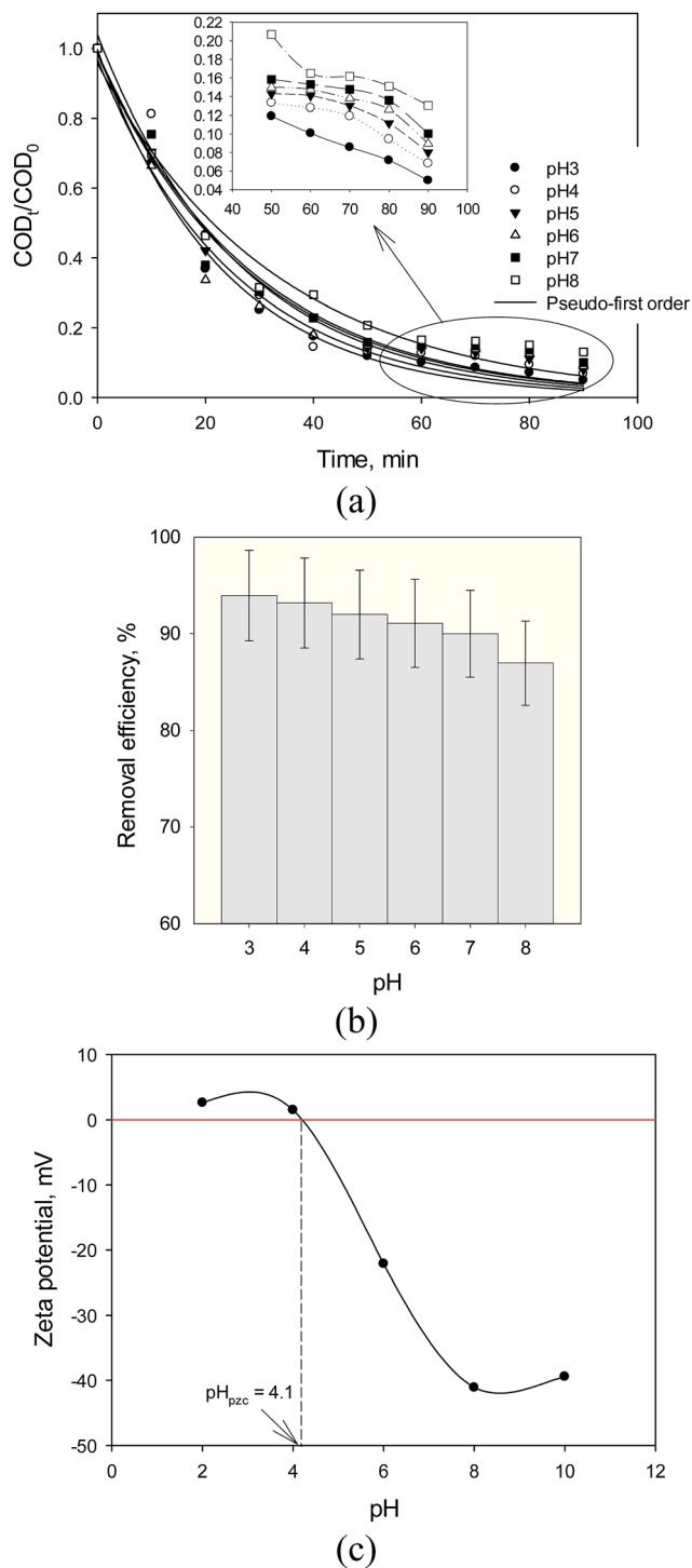
Fig. 9 (a) Kinetic curves, (b) removal efficiency of SMW with \text{Fe}_3\text{O}_4\text{@TiO}_2 (FT1) at different pH ( 1 \text{ g L}^{-1} photocatalyst dosage, 920 \text{ mg L}^{-1} initial COD, 90 min reaction time and 30^\circ\text{C} ) and (c) zeta potential and the pzc of \text{Fe}_3\text{O}_4\text{@TiO}_2 .
