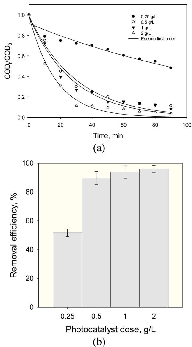
Fig. 10 (a) Kinetic curves, (b) removal efficiency of SMW with \text{Fe}_3\text{O}_4\text{@TiO}_2 (FT1) at different photocatalyst dose (pH = 3, 920 \text{ mg L}^{-1} initial COD, 90 min reaction time and 30^\circ\text{C} ).
