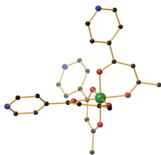
Fig. 1 The molecular structure of the fac -isomer of the metalloligand [M^{III}L_3] ( M = Fe, Cr, Al ). Colour code: M^{III} = \text{green} , O = red, N = blue, C = black. Hydrogen atoms have been omitted for clarity.
