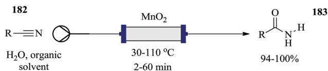
Fig. 25 Heterogeneous catalyzed continuous flow hydration of nitriles using manganese oxide.
