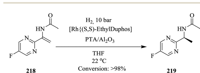
Scheme 43 Asymmetric hydrogenation in flow.
