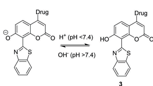
Fig. 3 A HBT-coumarin theranostic pH probe 3 for the monitoring of pH in cancer cells with UV activated drug release of chlorambucil. Measurement conditions: HEPES/ACN (7 : 3) buffer solution. Adapted with permission from ( J. Mater. Chem. B , 2015, 3 , 3490–3497). Copyright (2015) the Royal Society of Chemistry.
