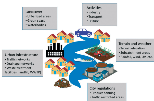
Fig. 1 Representation of the main factors influencing the emission of pollutants, including ENPs, in urban environments.
