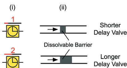
Fig. 10 (i) Symbolic and (ii) schematic representation of delay valves with dissolvable barriers. Arrow indicates flow direction.
