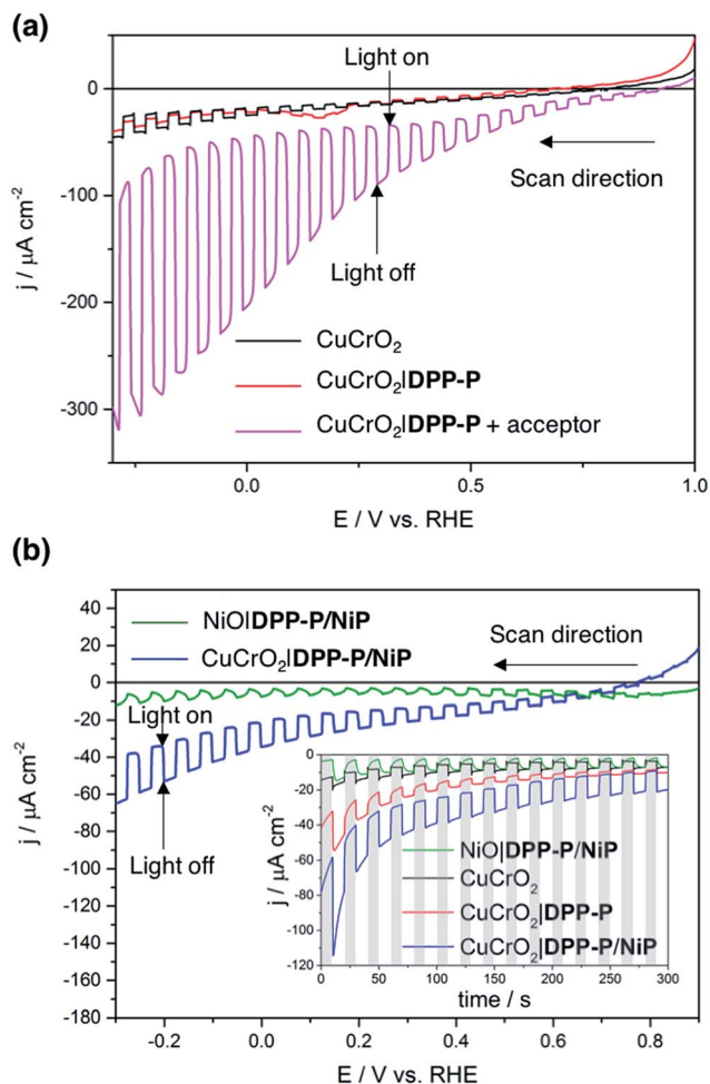
Fig. 3 Linear sweep voltammograms under chopped light illumination of (a) \text{CuCrO}_2 (black) and \text{CuCrO}_2|\text{DPP-P} (red) electrodes, and a \text{CuCrO}_2|\text{DPP-P} electrode with 5 mM DTDP acceptor in solution (magenta), (b) LSV scans of \text{CuCrO}_2|\text{DPP-P}/\text{NiP} (blue) and \text{NiO}|\text{DPP-P}/\text{NiP} (green) electrodes along with chronoamperograms (inset) of all relevant electrode compositions. The dark chops are shown with grey lines for the chronoamperograms. All experiments were performed in aqueous \text{Na}_2\text{SO}_4 electrolyte solution (0.1 M) adjusted to pH 3. Illumination with 100 \text{ mW cm}^{-2} , AM 1.5G, with a 420 nm cutoff filter at room temperature. An active electrode area of 0.25 \text{ cm}^2 was used with a scan rate of 5 \text{ mV s}^{-1} for voltammograms.
