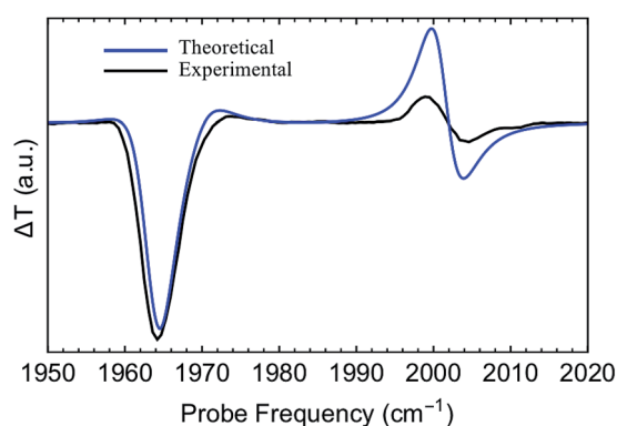
Fig. 9 Experimental and theoretical pump-probe (differential) transmission spectra of strongly coupled \text{W(CO)}_6 in an optical microcavity. 57 These results correspond to the case where the cavity photon and the molecular vibration (asymmetric C=O stretch) are resonant.
