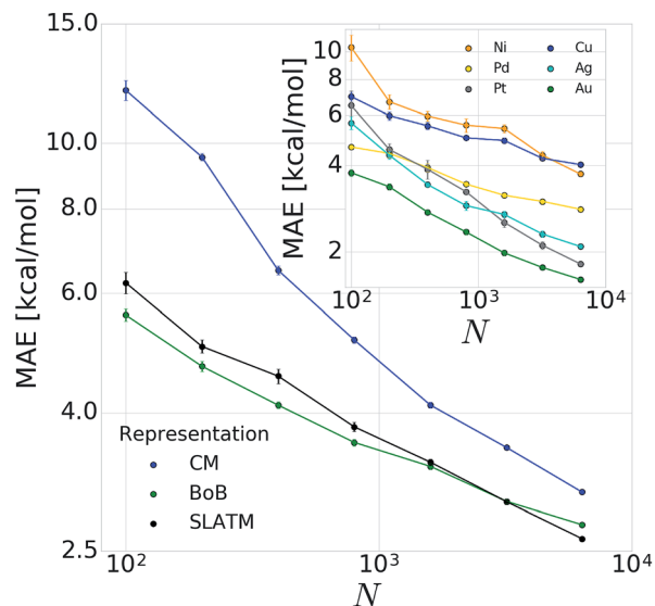
Fig. 4 Learning curves (test error of catalytic descriptor values as a function of training set size ( N )) for oxidative addition of vinyl bromide. Error bars correspond to standard deviation in cross validation. Inset: corresponding learning curves for individual metals for BoB.
