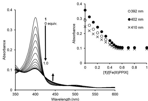
Fig. 5 UV-Vis titration of Fe(III)PPIX (2.4 \mu M) with 1 in DMSO/33 mM HEPES buffer (pH 7.4) = 2 : 3 (v/v) at 25 ^{\circ} C. Inset: changes in the absorbance of Fe(III)PPIX upon the addition of 1 .
