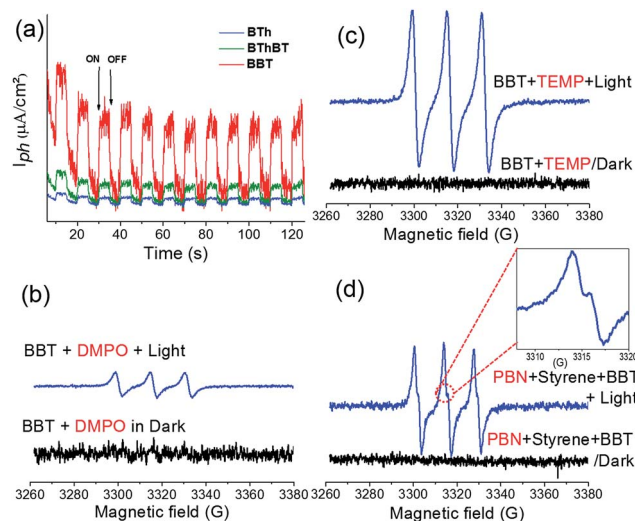
Fig. 4 (a) Photocurrent responses of the CMPs under the illumination of visible light with a wavelength \geq 420 nm with a light ON/OFF model. EPR spectra of (b) DMPO- \text{O}_2^{\cdot-} ( g = 2.00639 ) and (c) TEMP- ^1\text{O}_2 adducts ( g = 2.00645 ) using BBT as the photocatalyst in the dark and under light irradiation ( \lambda = 460 nm, 0.065 \text{ W cm}^{-2} ). (d) EPR spectra using PBN as a radical trapping agent for the radical intermediate of styrene, with BBT, under \text{O}_2 and light irradiation ( g = 2.00667 ).
