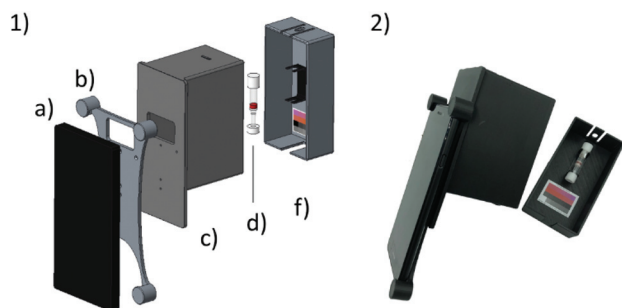
Fig. 2 Illustration of the imaging system: (1) isometric view with (a) smartphone with app, (b) smartphone holder, (c) case, (d) CyanoKit sensing cartridge, (e) cap with cartridge holder and colour calibration chart of prototype used for experimentation. (2) Photograph of whole system that was used for experimentation.
