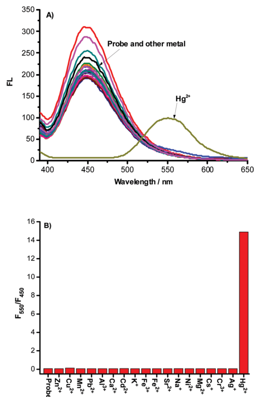
Fig. 2 (A) Fluorescence spectra of probe NAP-PS (10 \mu M) before and after the addition of 200 \mu M different metal ions in HEPES buffer (1.0 mM, pH = 7.4), \lambda_{\text{ex}} = 380 nm, slits: 3/5 nm; (B) fluorescence intensity ratios ( F_{550}/F_{450} ) of probe NAP-PS (10 \mu M) before and after the addition of 200 \mu M different metal ions in HEPES buffer (1.0 mM, pH = 7.4).
