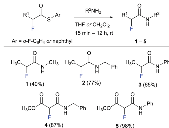
Scheme 1 Synthesis of \alpha fluoro amides 1–5.
