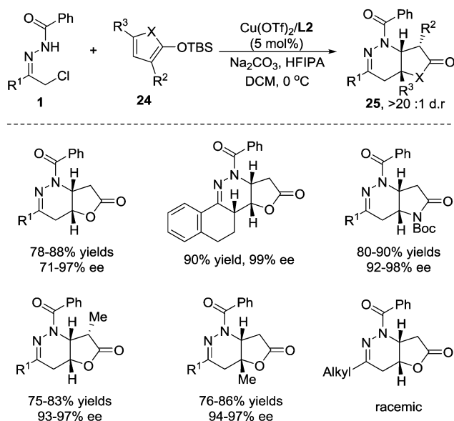
Scheme 10 Cu(II)/tBu-Box catalyzed formal [4+2] annulation of azoalkene with 2-silyloxyfuran.
