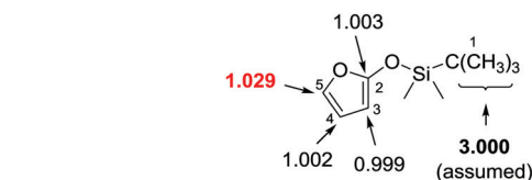
Scheme 11 Carbon isotope effects (R/R 0 ) calculated for TBSOF furan. The three methyl carbons of the tBu group (in bold) were taken as the internal standard.
