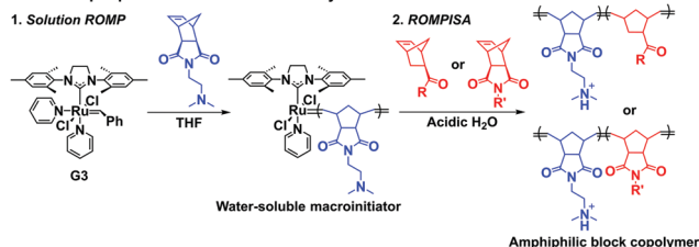
Scheme 2 Reported synthetic strategies to conduct aqueous dispersion ROMPISA for fabrication of diblock copolymer nano-objects of various morphologies. (A) One-pot aqueous ROMPISA mediated by a water-soluble HG2 catalyst, and (B) two-step aqueous ROMPISA mediated via a water-soluble PNB macroinitiator prepared in organic solvent using G3 .
